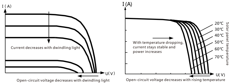
Fig. 1-3 Relation between solar panel output characteristics and illumination
