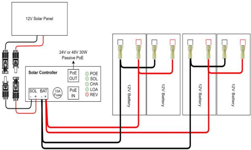
12V Battery Configuration
