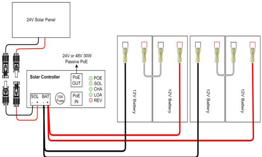
24V Battery Configuration
