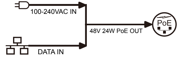
Passive PoE Injector TP-POE-48
