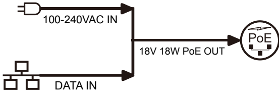
GigE Passive PoE Injector TP-POE-18G
