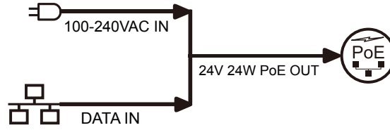
Passive PoE Injector TP-POE-24
