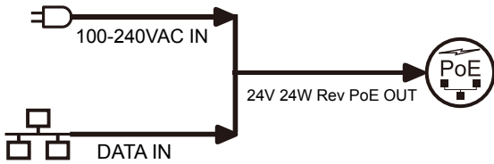
Passive PoE Injector TP-POE-24IR-CI
