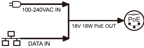
Passive PoE Injector TP-POE-18
